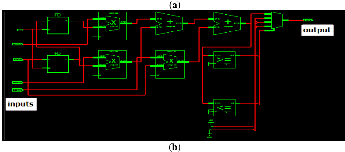
Fig. 7 (a) Time diagram , (b) hardware circuit, of implementing neuron with satlins activation function.
