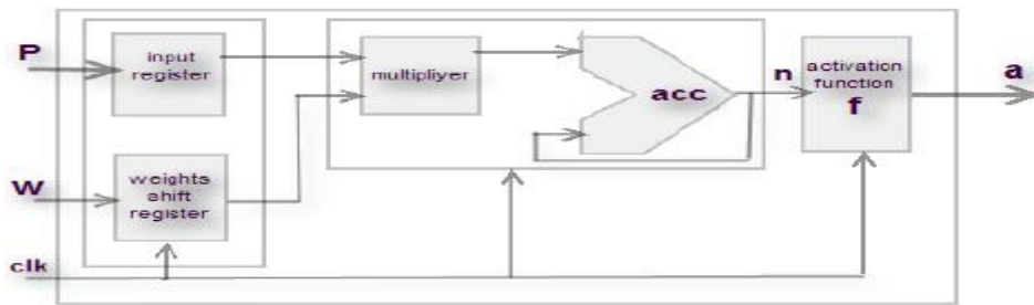
Fig.( 2 ) VHDL structural diagram for neuron implementation.
