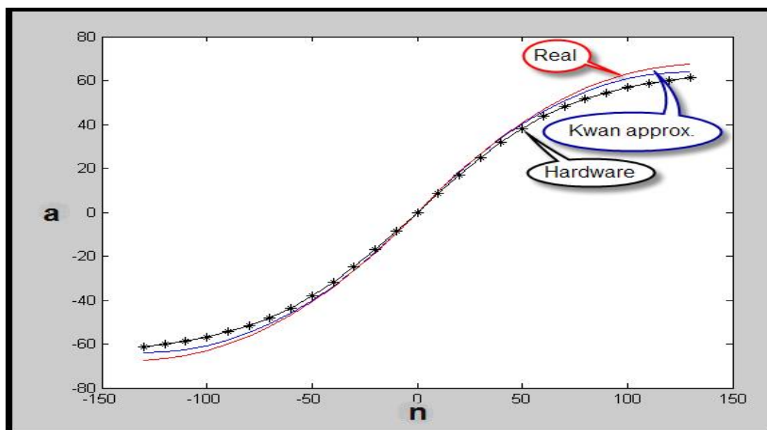
Fig. ( 11 ) Tansig activation function hardware results.
