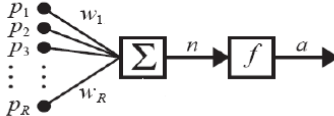
Fig.( 1) mathematical model of artificial neuron .
