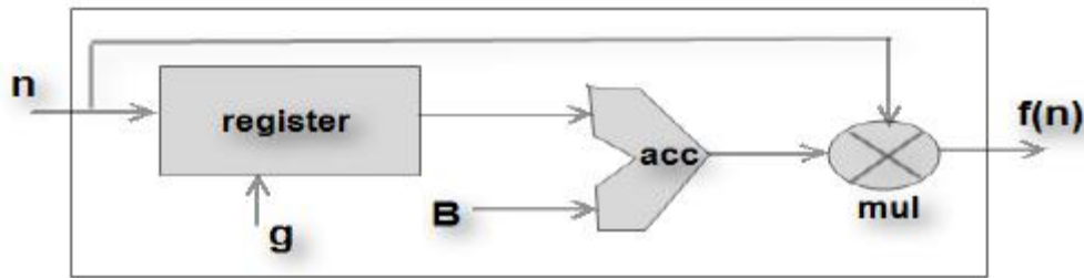
Fig. ( 9 ) block diagram of the tansig activation function implementation.
